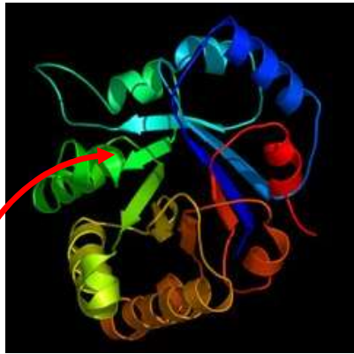
Triosephosphateisomerase "TIM"
