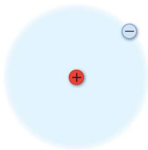
Protium 1 proton 0 neutrons
