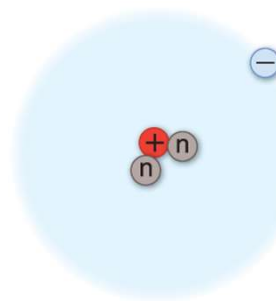
Tritium 1 proton 2 neutrons
